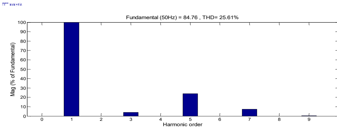
Figure 9 THD for Load Current
