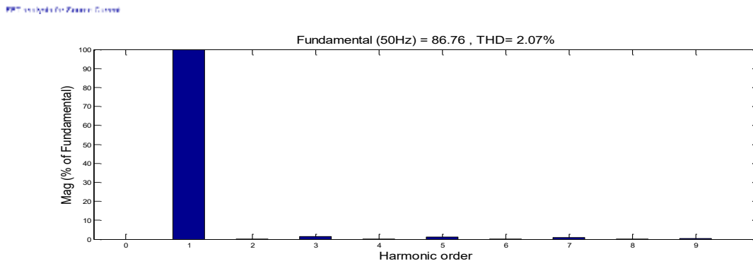
Figure 10 THD For Grid Current with Cuckoo based Fuzzy controller
