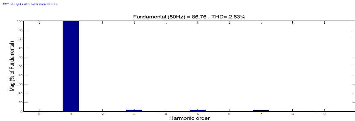
Figure 10 THD For Grid Current with Cuckoo based Fuzzy controller
